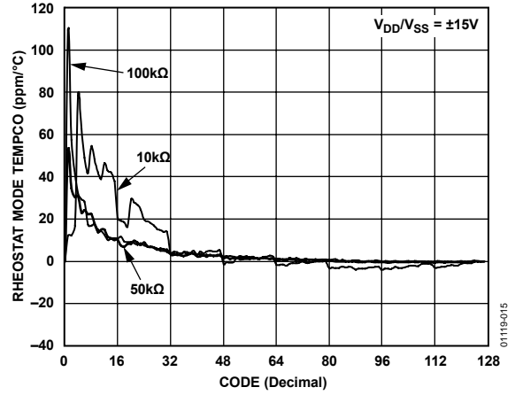
Figure 15. (\Delta V_{WB}/V_{WB})/\Delta T Potentiometer Mode Tempo
