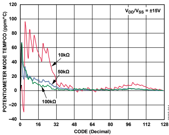
Figure 14. (\Delta R_{WB}/R_{WB})/\Delta T Rheostat Mode Tempo
